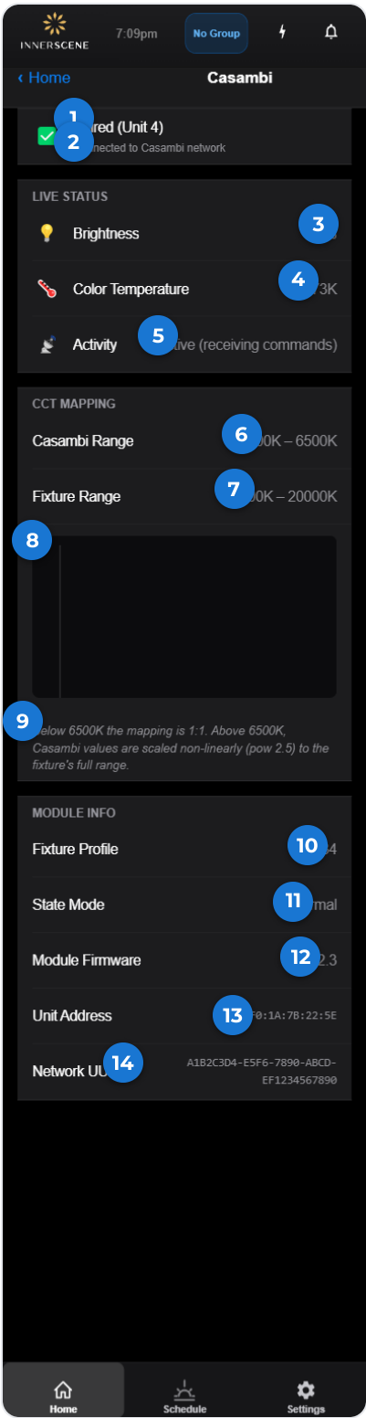
Status and configuration page for a fixture equipped with a Casambi daughterboard. Shows pairing status with the Casambi network, live brightness/CCT readings from the wireless mesh, the CCT mapping curve between Casambi values and the fixture's range, and module identification info.
